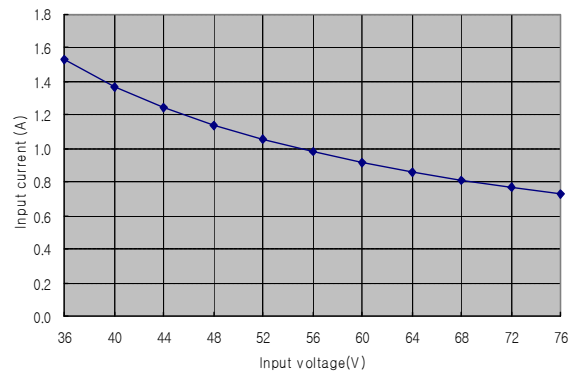
Input current vs input voltage
