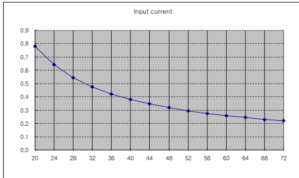
Vin=48V, Vo=3.3V@4A, At 25°C
