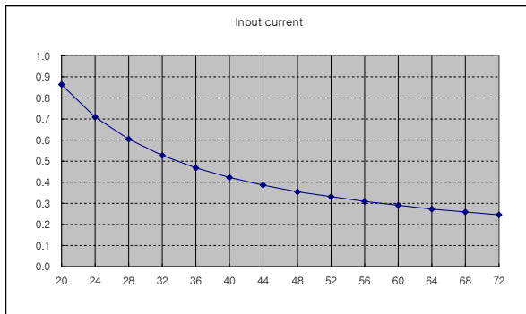
Vin=48V, Vo=5V@3A, At 25°C
